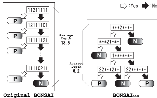
Fig. 6. Typical decision trees from the original BONSAL and BONSAL iiS . The left tree has been selected from decision trees obtained by the original BONSAL and the right one obtained by BONSAL iiS .
