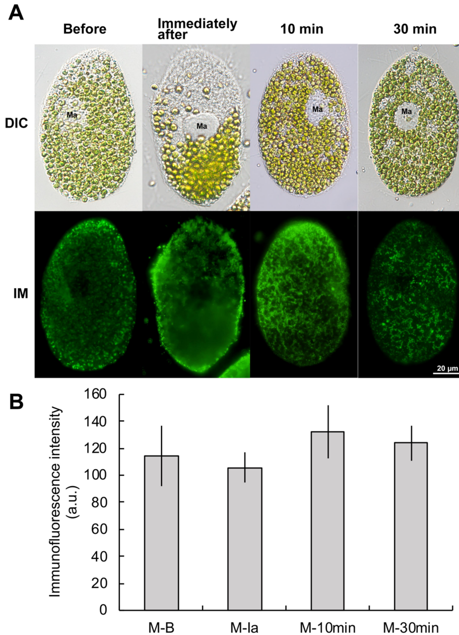
Figure 3. (A) Indirect immunofluorescence micrographs of the high-speed centrifuged algae-bearing Paramecia with the monoclonal antibody against mitochondria.
