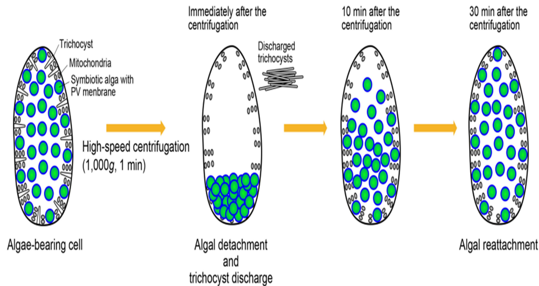
Figure 5. A schematic diagram of changes in localization of symbiotic algae with PV membrane, host mitochondria, and trichocysts before and after high-speed centrifugation. Before the centrifugation, numerous host mitochondria and trichocysts are attached beneath the host cell cortex, with symbiotic algae settled between them. After the centrifugation, the symbiotic algae detach from the host cell cortex, immediately accumulating at the posterior end of the host cell. At the same time, almost all trichocysts are released out of the cell, but mitochondria remain anchored. The symbiotic algae gradually reattach by host cytoplasmic streaming, which is complete within 30 min. At that time, the algae attach between mitochondria, but trichocysts are not required for the algal attachment.
