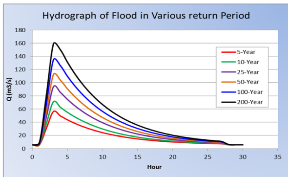
Figure 3 Hydrograph of Flood in various return periods.
