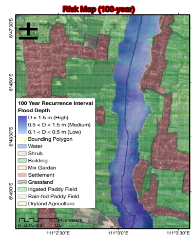
Figure 8 Risk map (100-year).
