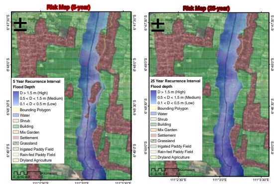
Figure 7 Risk map (Left:5-year and Right:25-year).
