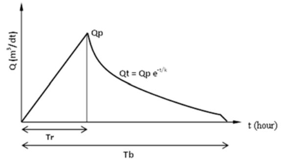
Figure 2 The concept of SUH GAMA I
