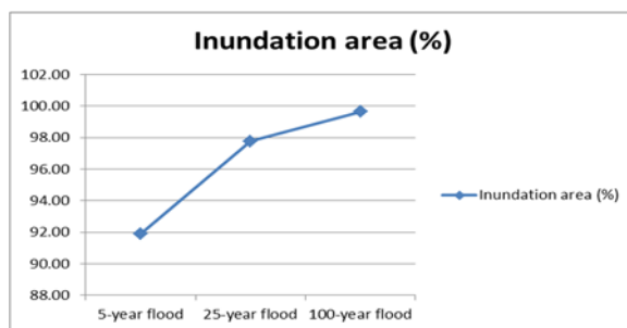
Figure 6. Percentage of inundation area.
