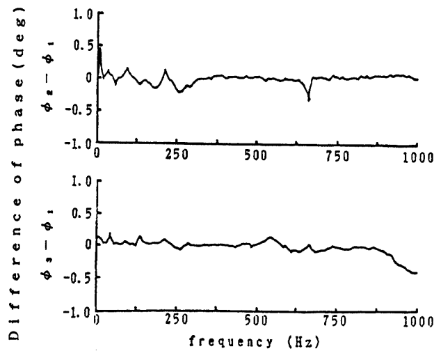
Fig. 6 Magnitude and phase difference between two channels
