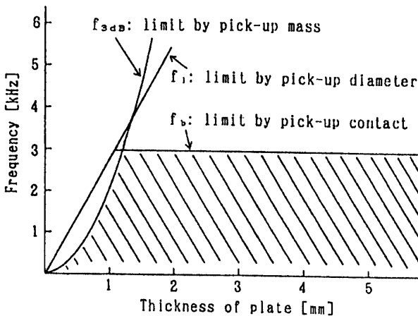
Fig. 5 Frequency ranges of application for the three channel pickup
