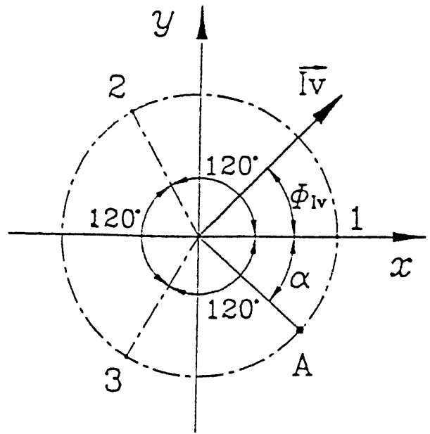
Fig. 2 Arrangement of vibration transducers for the three channel method
