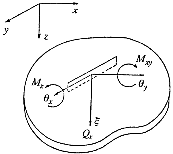
Fig. 1 Force and moments affect a small cross-section in plate
