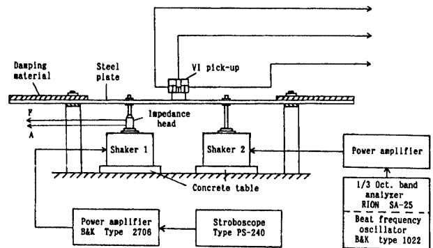
Fig. 7 Schematic of experimental setup
