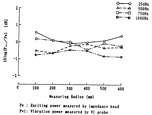
Fig.12 Difference of excited power and vibrated power
