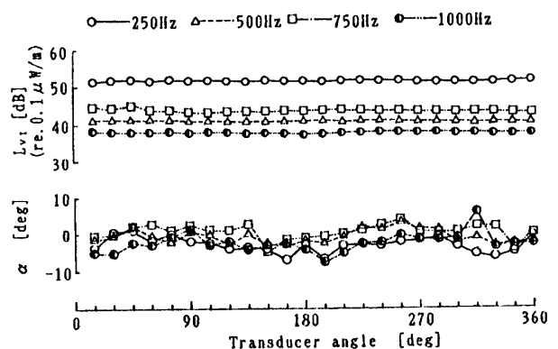
Fig. 9 Deviation of the VI pickup in magnitude and direction
