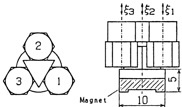
Fig. 3 VI pickup for three channel method
