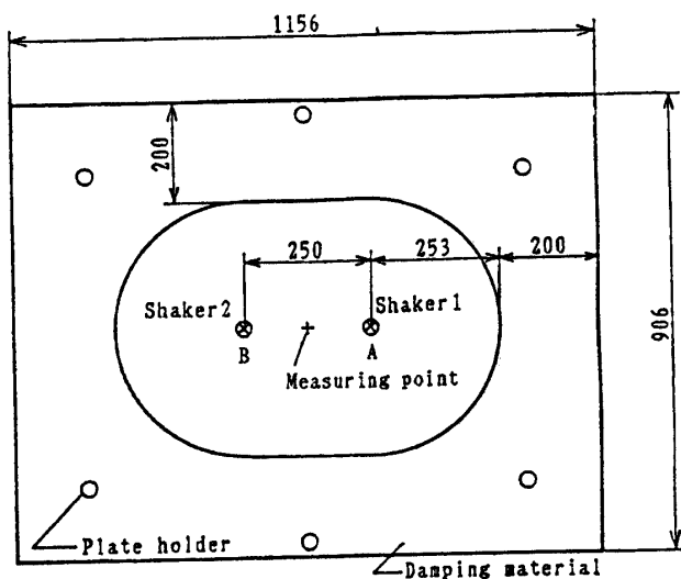
Fig. 8 Tested plate for examining directional characteristic of VI pickup
