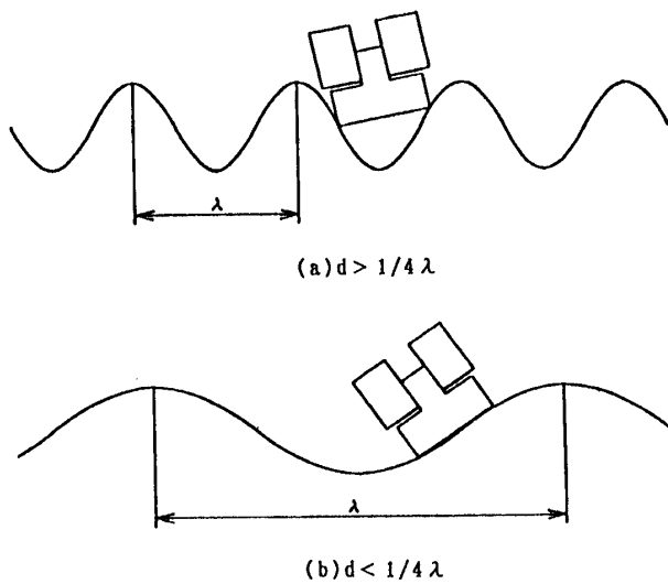
Fig. 4 Behavior of VI pickup and flexural wave length
