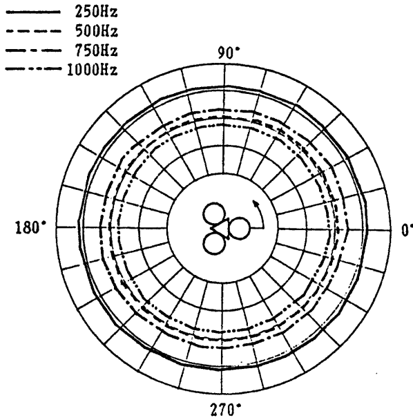
Fig.10 Directional distributions of VI level
