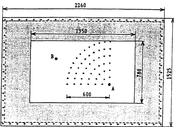
Fig.11 Tested plate for measuring vibration power
