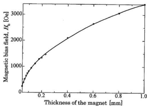
Fig. 4 Relationship between magnetic bias field in center of YIG single crystal and thickness of permanent magnet obtained by calculation.
