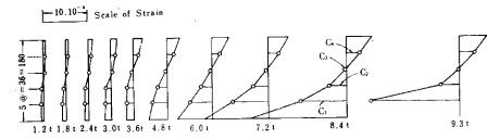
Fig.11 a, b Case of specimen B
