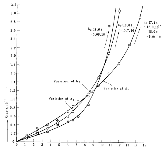
Fig.14 a, b Case of specimen B
