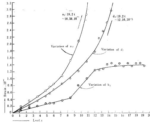
Fig.13 a, b Case of specimen A
