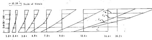
Fig.13 a, b Case of specimen A
