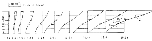
Fig.14 a, b Case of specimen B
