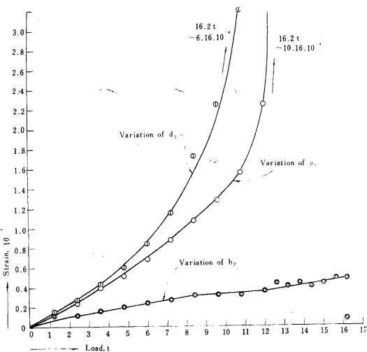
Fig.10, 11, 12 Strains of under reinforced concrete deformed steel bar beam
