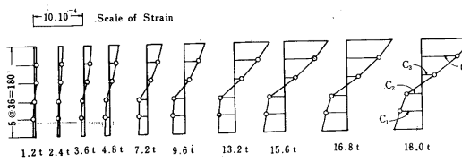
Fig.15 a, b Case of specimen C
